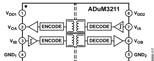
Figure 2. ADuM3211
