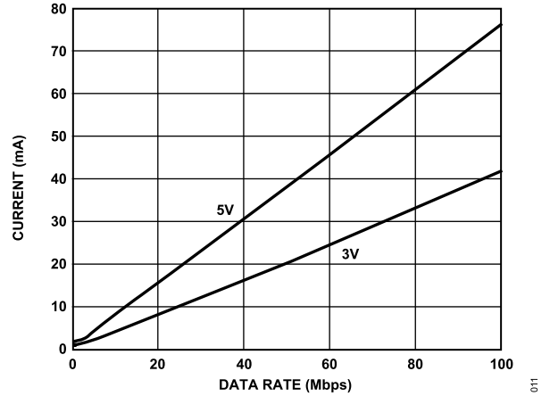
Figure 11. Typical ADuM2400 V DD1 Supply Current vs. Data Rate for 5 V and 3 V Operation
