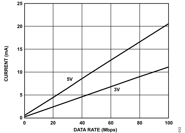
Figure 12. Typical ADuM2400 V DD2 Supply Current vs. Data Rate for 5 V and 3 V Operation
