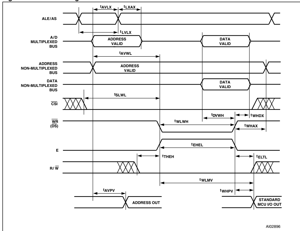
Figure 48. WRITE Timing
