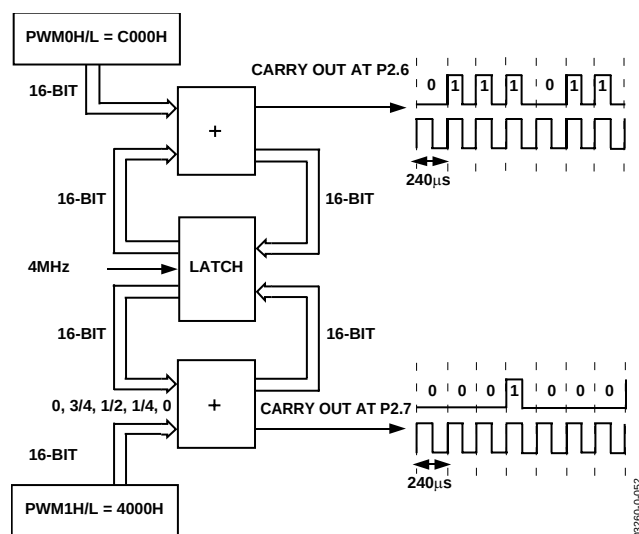
Figure 53. PWM Mode 6
