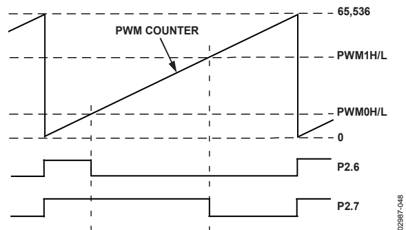
Figure 59. PWM Mode 3
