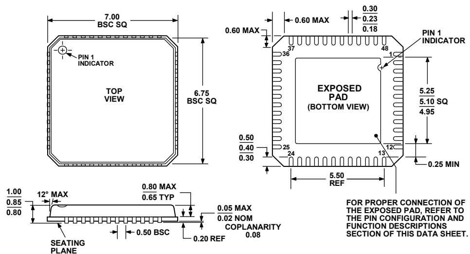
Figure 61. 48-Lead Lead Frame Chip Scale Package [LFCSP_VQ]
