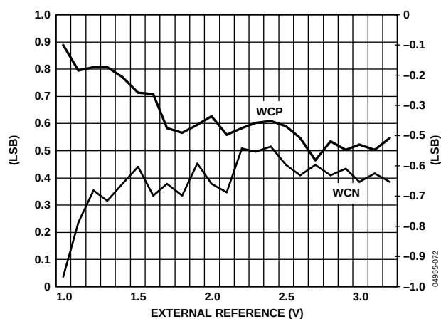
Figure 30. Typical Worst-Case (Positive (WCP) and Negative (WCN)) INL Error vs. V_{REF} , f_s = 774 \text{ kSPS}
