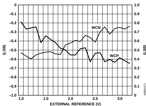
Figure 33. Typical Worst-Case (Positive (WCP) and Negative (WCN)) DNL Error vs. V_{REF} , f_s = 774 \text{ kSPS}
