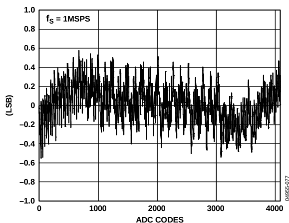
Figure 29. Typical INL Error, f_s = 1 \text{ MSPS}
