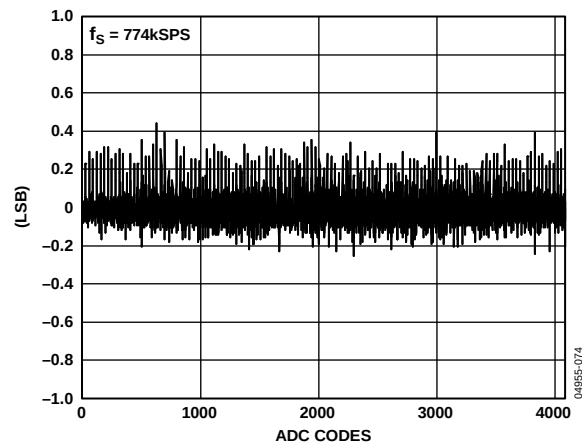
Figure 31. Typical DNL Error, f_s = 774 \text{ kSPS}
