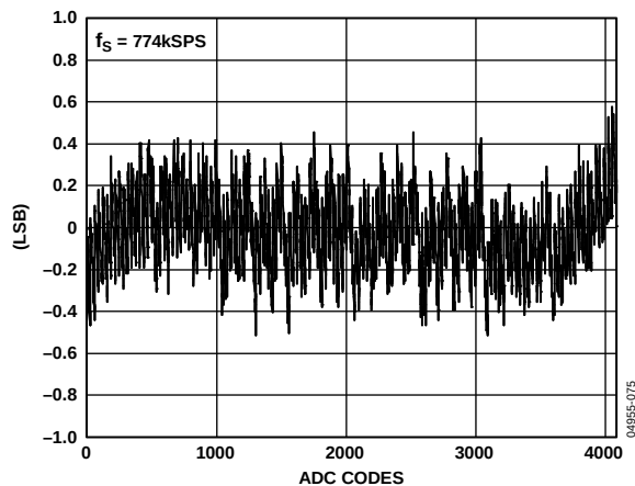
Figure 28. Typical INL Error, f_s = 774 \text{ kSPS}
