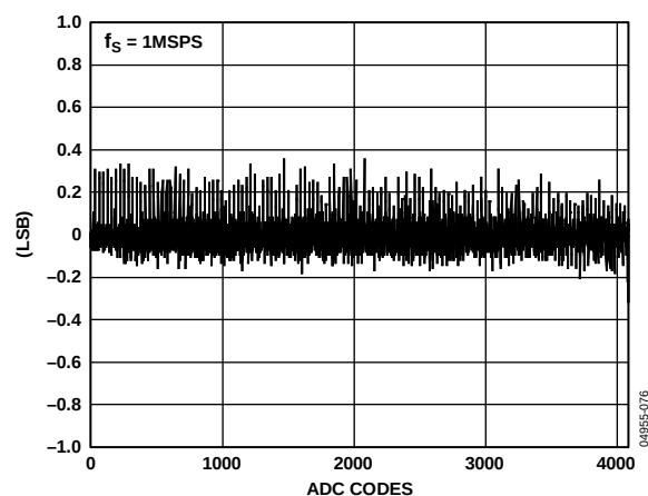
Figure 32. Typical DNL Error, f_s = 1 \text{ MSPS}
