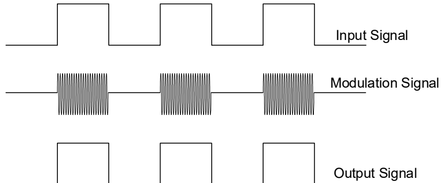
Figure 2. Modulation Scheme
