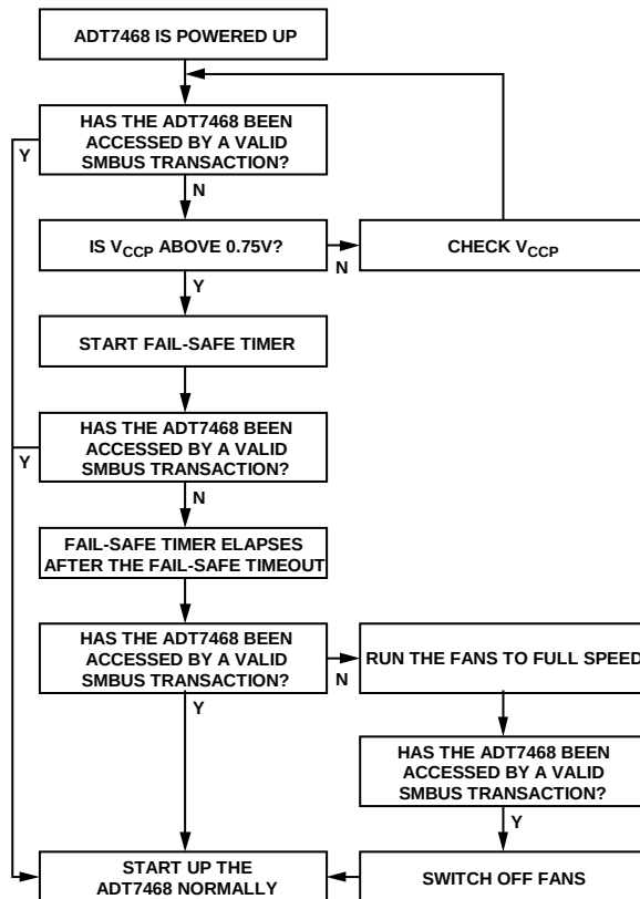
Figure 48. Power-On Flow Chart
