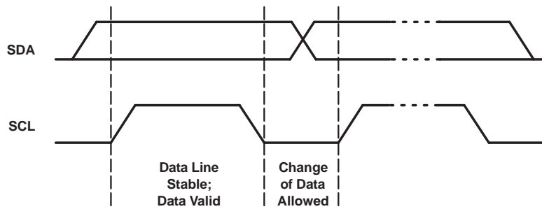
Figure 20. Bit Transfer
