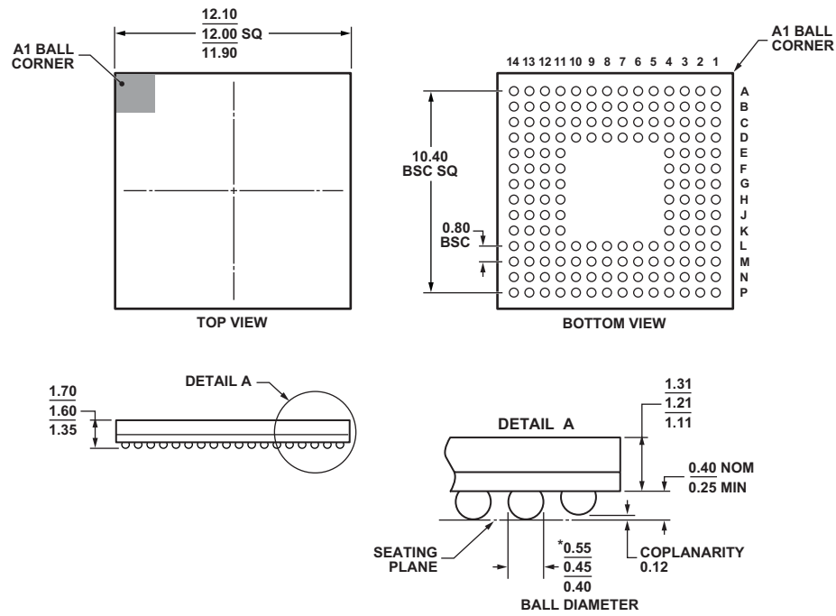
Figure 65. 160-Ball Chip Scale Package Ball Grid Array [CSP_BGA] (BC-160-2) Dimensions shown in millimeters
