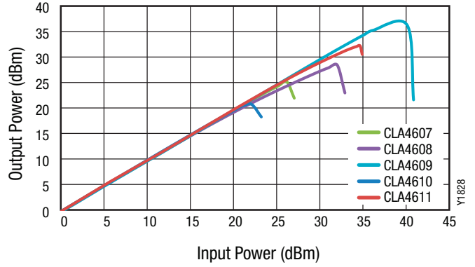
Figure 2. CLA4607 to CLA4611 CW Output vs Input Power
