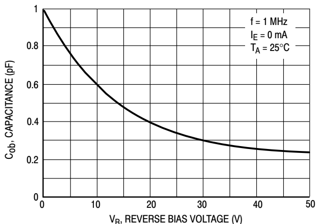
Figure 28. Output Capacitance
