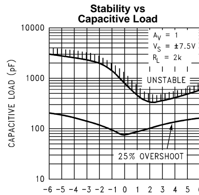
V_{OUT} (V) Figure 50.
