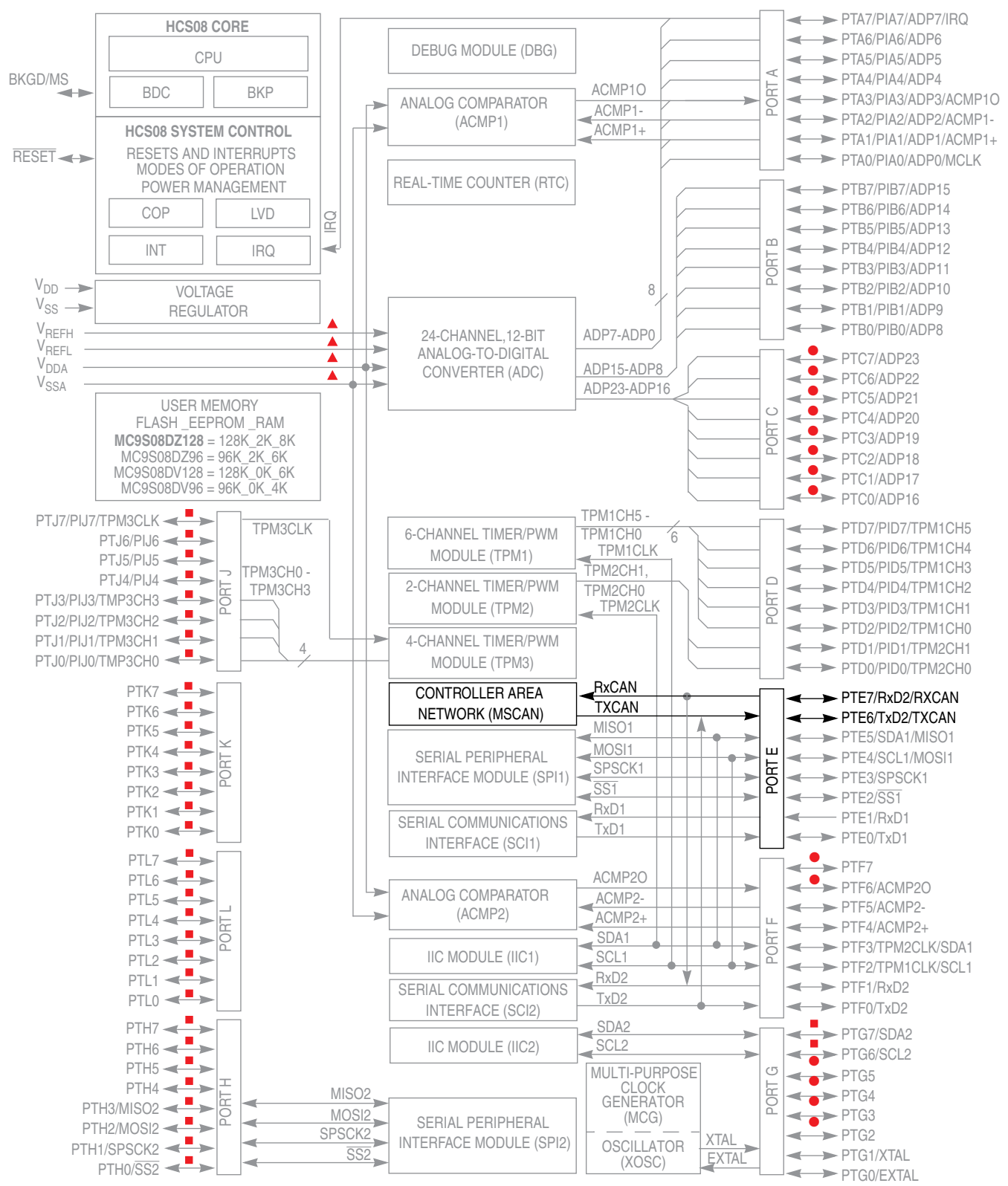
■ - Pin not connected in 64-pin and 48-pin packages ● - Pin not available in the 48-pin package ▲ - In 48-pin package, VDDA and VREFH are internally connected to each other and VSSA and VREFL are internally connected to each other.
