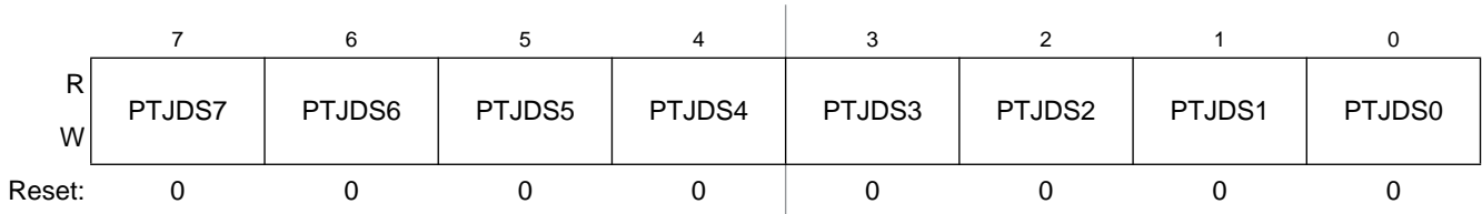
Figure 6-56. Drive Strength Selection for Port J Register (PTJDS)
