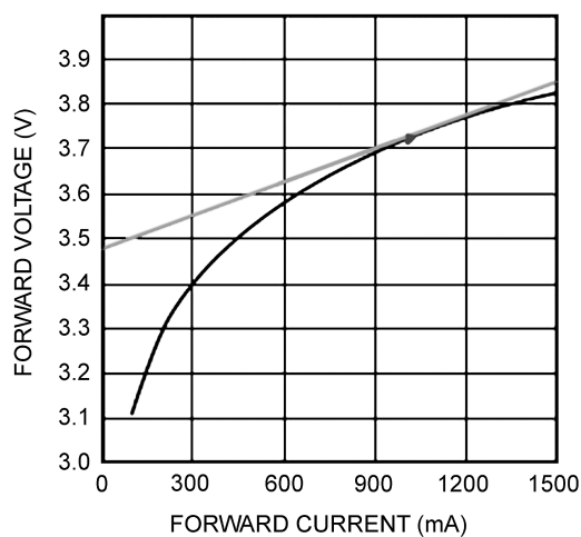
Figure 25. Dynamic Resistance
