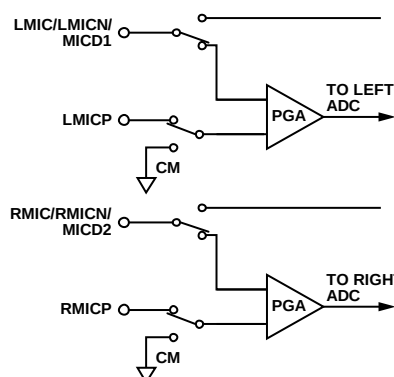
Figure 33. Differential Input Configuration
