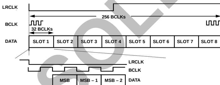
Figure 49. TDM Mode
