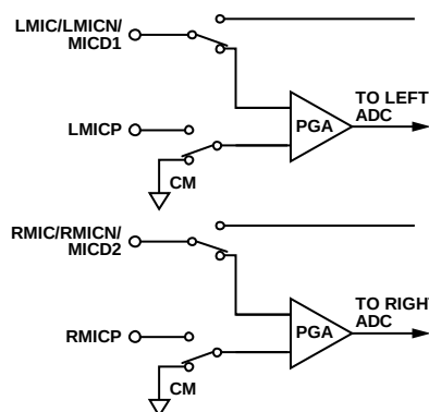
Figure 32. Single-Ended Input Configuration
