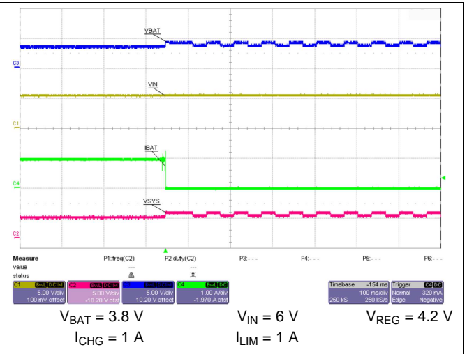
Figure 2. Battery Removal
