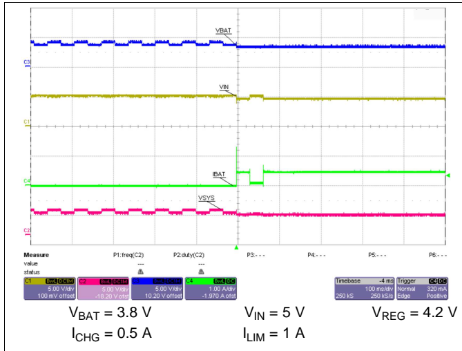
Figure 1. Battery Detection
