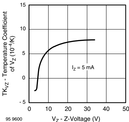
Fig. 3 - Temperature Coefficient of V_Z vs. Z-Voltage
