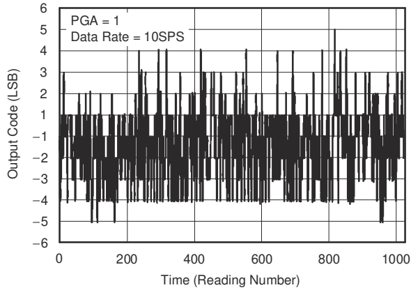
Figure 6-1. Noise Plot
