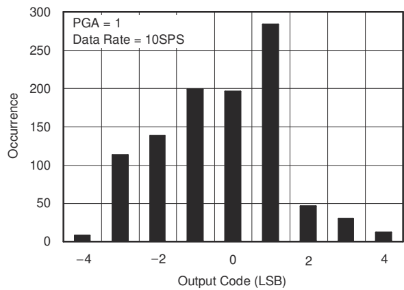
Figure 6-1. Noise Plot
