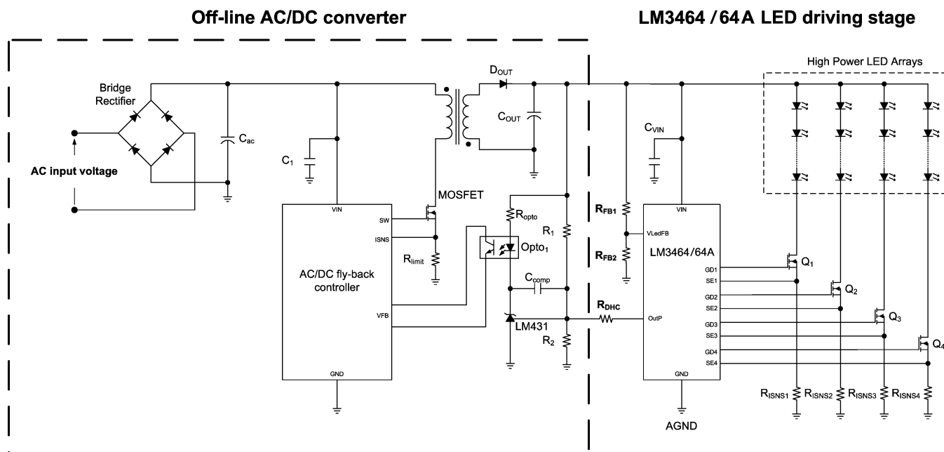
Figure 14. Typical Application Circuit with Fly-Back AC/DC Converter
