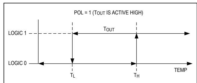
Figure 5. Thermostat Output Operation
