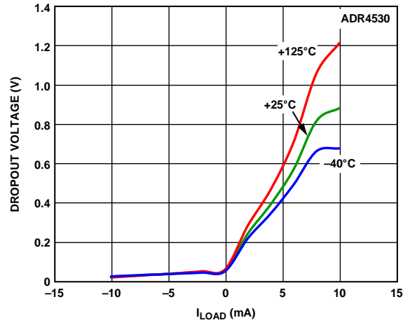
Figure 33. ADR4530 Dropout Voltage vs. Load Current
