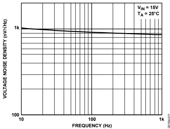
Figure 11. Voltage Noise Density vs. Frequency
