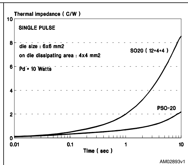
Figure 14. PowerSO-20: with external heatsink Figure 15. Thermal impedance of PowerSO-20 and standard SO20
