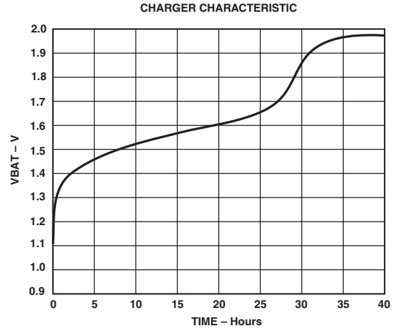
Figure 10. Seiko TS621 Charge Characteristic
