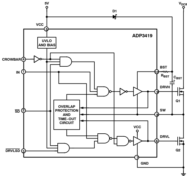
Figure 16. Detailed Block Diagram of the ADP3419
