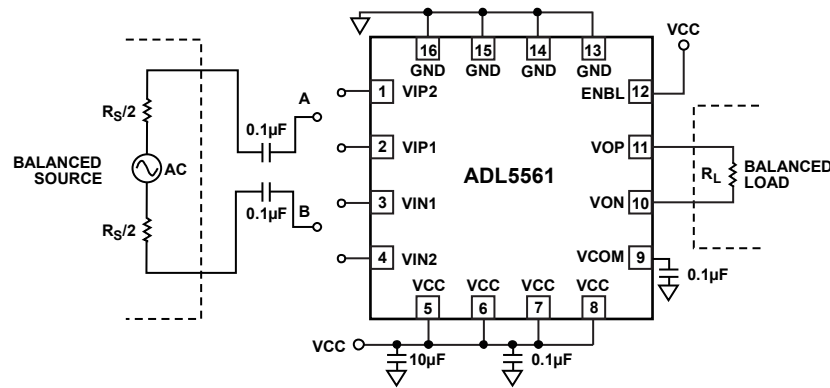
Figure 33. Basic Connections
