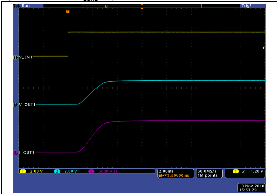
Figure 23. Turn-on for C_{LOAD} = 1\ \mu\text{F}
