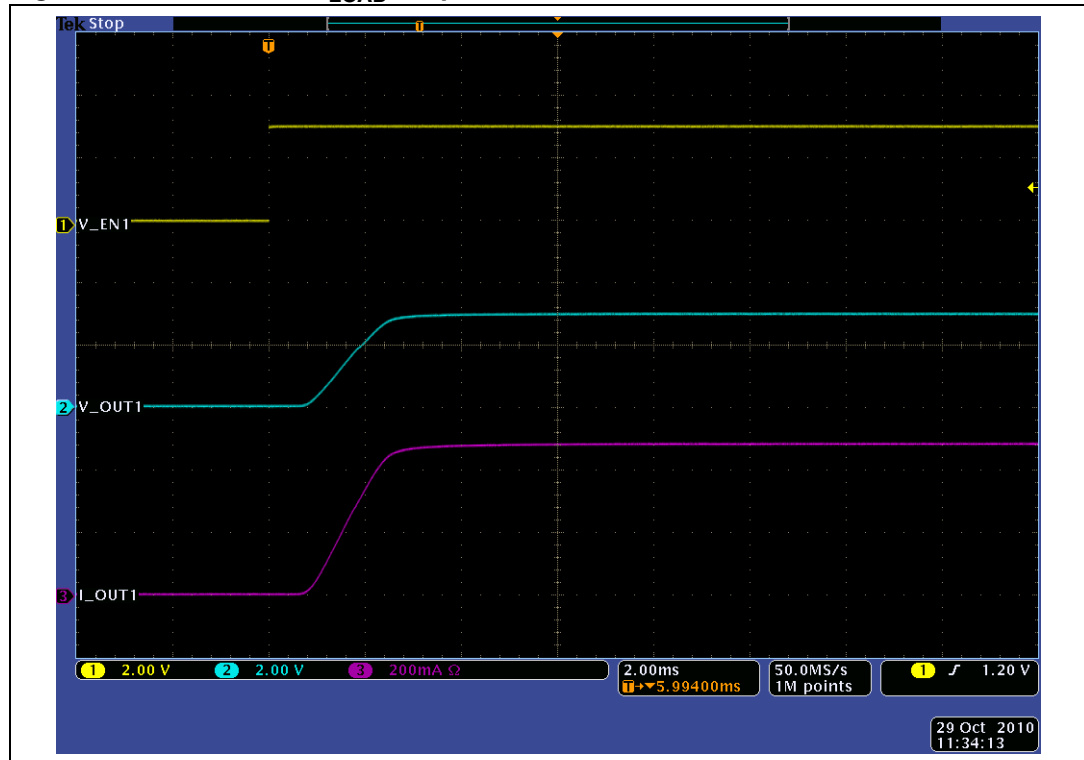
Figure 3. Turn-on for C_{LOAD} = 1\ \mu\text{F}
