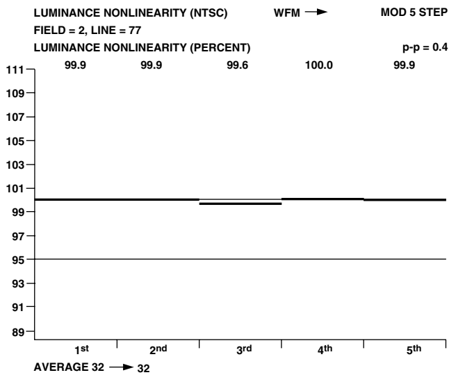
Figure 136. NTSC Luminance Nonlinearity
