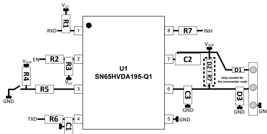
Figure 10-4. Layout Example
