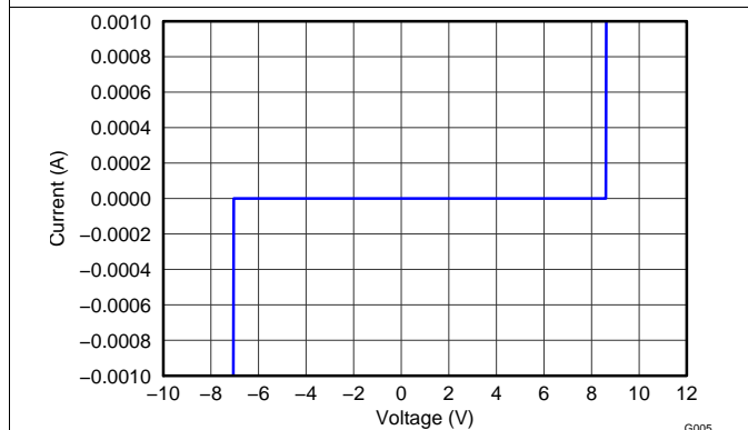
Figure 5. IV Curve
