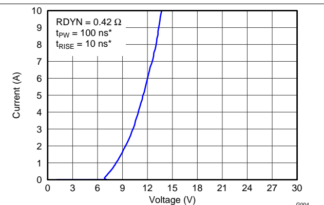
Figure 4. TLP, t_{PW} = 100 \text{ nS} , t_{RISE} = 10 \text{ nS} , GND to Data
