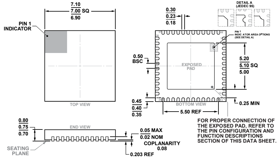
Figure 14. 48-Lead Lead Frame Chip Scale Package [LFCSP] 7 mm × 7 mm Body and 0.75 mm Package Height (CP-48-4) Dimensions shown in millimeters
