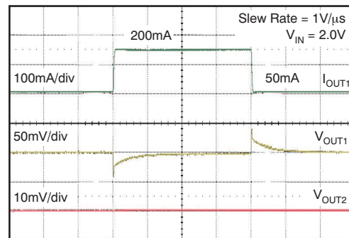
Time (50 \mu\text{s} /div) Figure 62.
