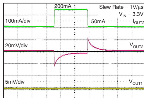
Time (50 \mu\text{s} /div) Figure 64.
