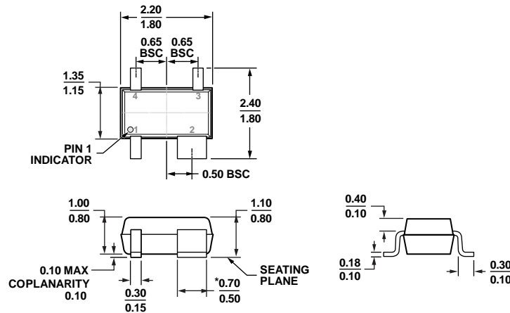
*PACKAGE OUTLINE CORRESPONDS IN FULL TO EIAJ SC82 EXCEPT FOR WIDTH OF PIN 2 AS SHOWN. Figure 16. 4-Lead Thin Shrink Small Outline Transistor Package [SC70] (KS-4) Dimensions shown in millimeters
