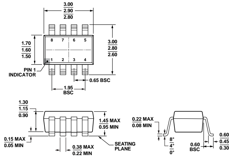
Figure 50. 8-Lead Small Outline Transistor Package [SOT-23] (RJ-8)
