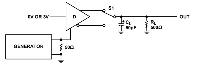
Figure 9. Driver Propagation Delays
