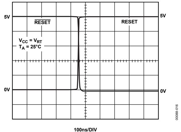
Figure 10. \overline{RESET} , RESET Assertion
