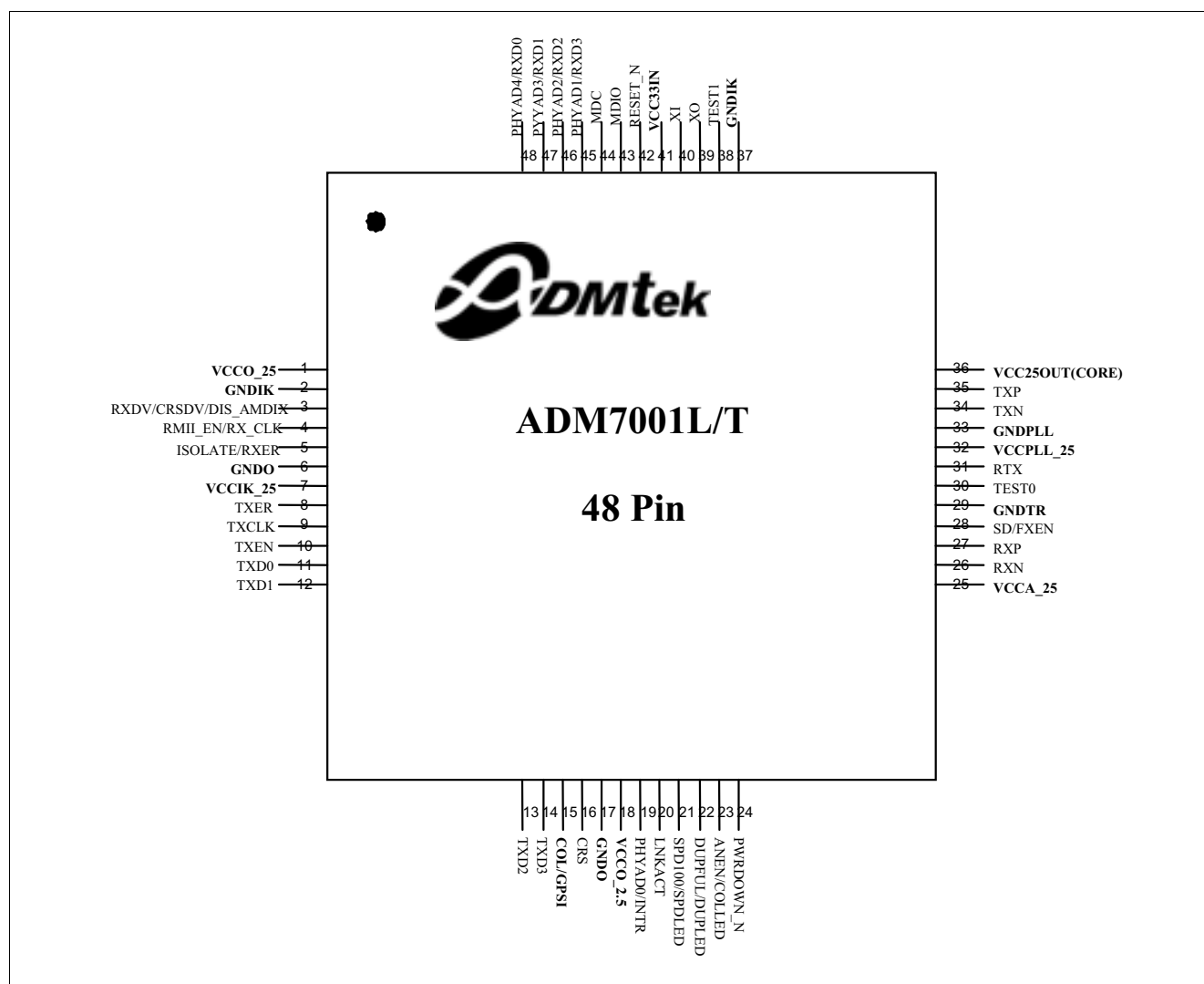
Figure 2 Pin Diagram
