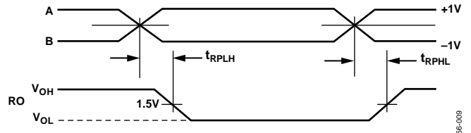
Figure 24. Receiver Propagation Delays
