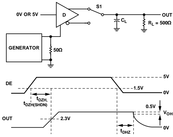
Figure 21. Driver Enable and Disable Times ( t_{DZH} , t_{DZH(SHDN)} , t_{DZH} , t_{DZH(SHDN)} )
