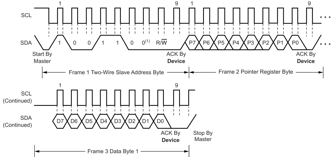
Figure 7-4. Two-Wire Timing Diagram for Write Word Format
