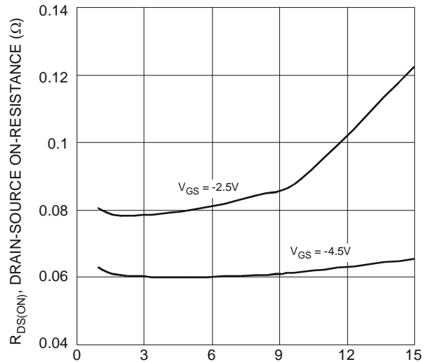
Figure 14 Typical On-Resistance vs. Drain Current and Gate Voltage
