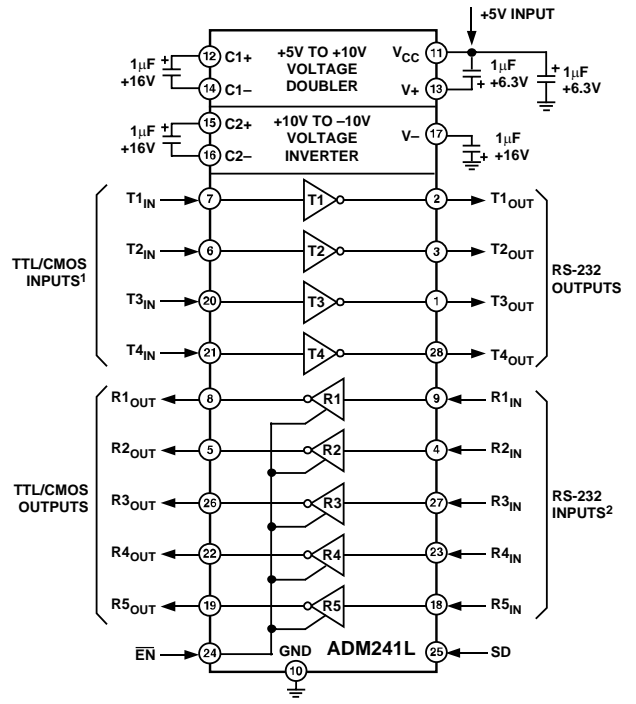
1INTERNAL 400kΩ PULL-UP RESISTOR ON EACH TTL/CMOS INPUT. 2INTERNAL 5kΩ PULL-DOWN RESISTOR ON EACH RS-232 INPUT.
