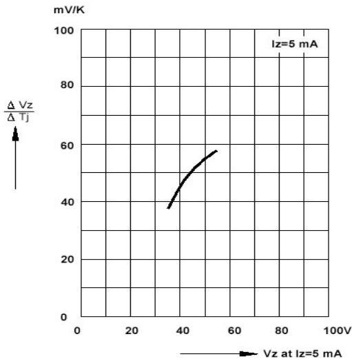
Figure 13. Temperature Dependence of Zener Voltage vs. Zener Voltage
