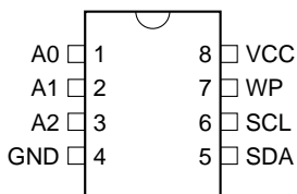
8-Pin PDIP
