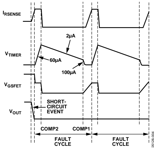
Figure 40. ADM1172-1 Automatic Retry During Overcurrent Fault
