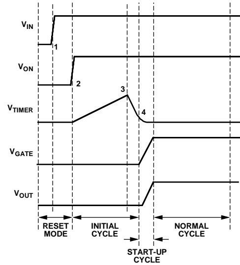
Figure 36. Power-Up Timing
