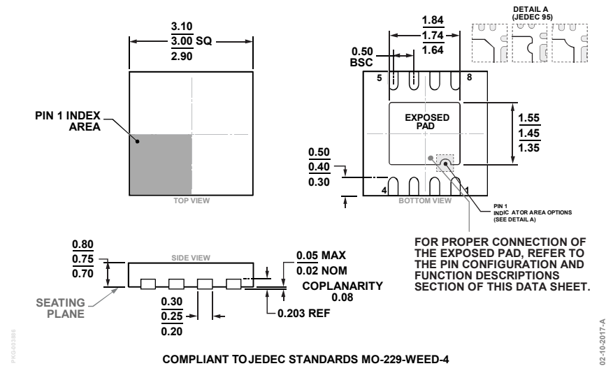
Figure 65. 8-Lead Lead Frame Chip Scale Package [LFCSP] 3 mm × 3 mm Body and 0.75 mm Package Height (CP-8-13) Dimensions shown in millimeters
