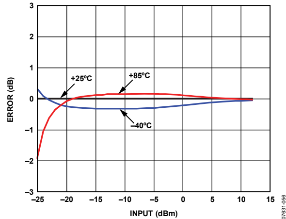
Figure 56. VRMS Error from +25^{\circ}\text{C} Output Voltage at -40^{\circ}\text{C} , +25^{\circ}\text{C} , and +85^{\circ}\text{C} After Ambient Normalization, Frequency 1900 MHz, Supply 3.0 V
