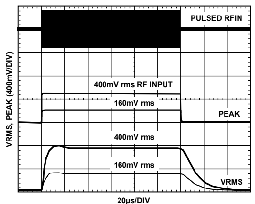
Figure 38. Output Response to Various RF Input Pulse Levels, Supply 3 V, 900 MHz Frequency, C_{FLTR} = 10 \text{ nF} , C_{OUT} = \text{Open}
