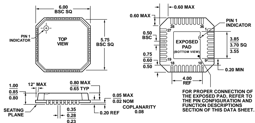
COMPLIANT TO JEDEC STANDARDS MO-220-VJJD-1 Figure 57. 36-Lead Lead Frame Chip Scale Package [LFCSP_VQ] 6mm × 6 mm Body, Very Thin Quad (CP-36-1) Dimensions shown in millimeters
